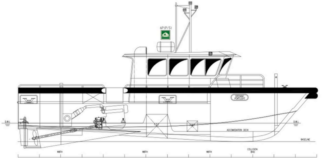
OUTBOARD PROFILE
