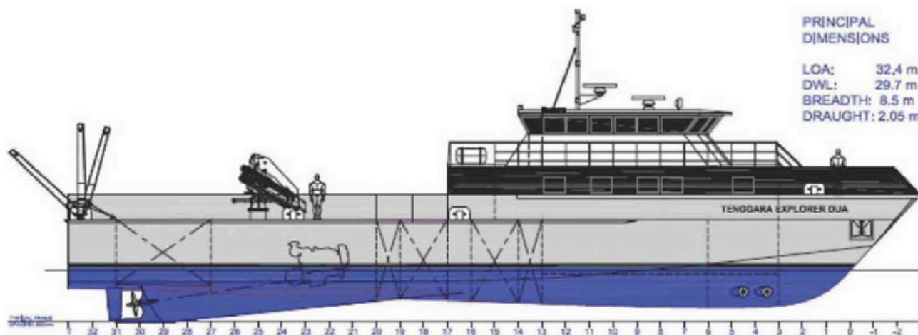
OUTBOARD PROFILE
