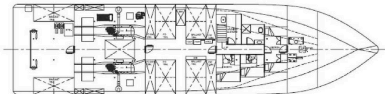
LOWER DECK
